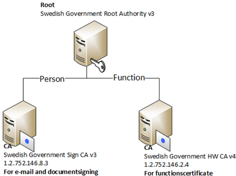
Figure 2 – Issuing CAs of the SSIA PKI
