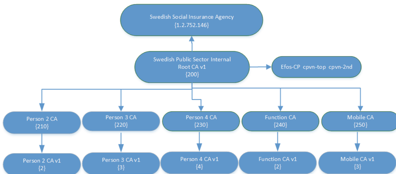
Figure 2 – EFOS PKI OID hierarchy
