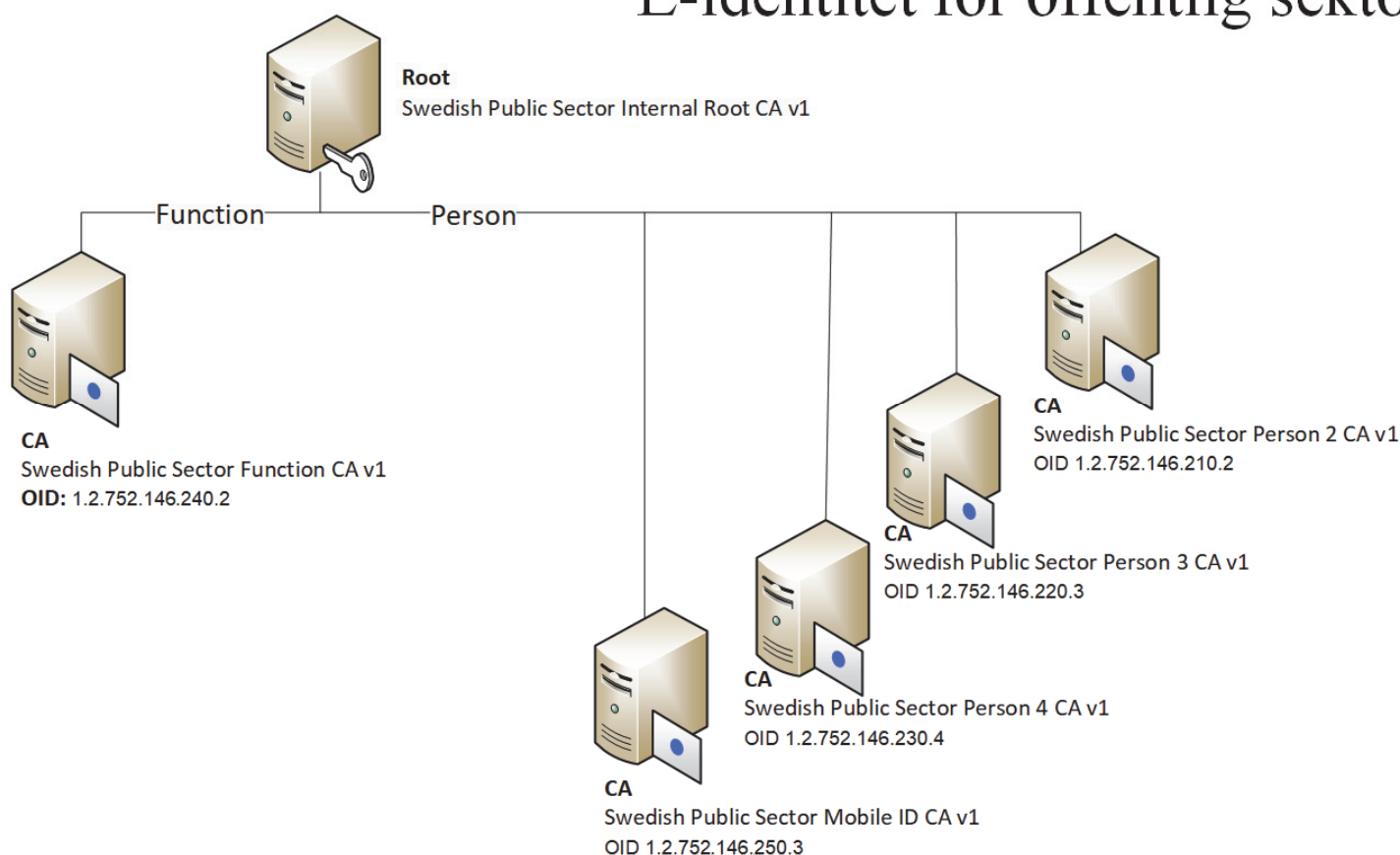
Figure 3 – EFOS PKI mapping between certificate OID's and assurance level
